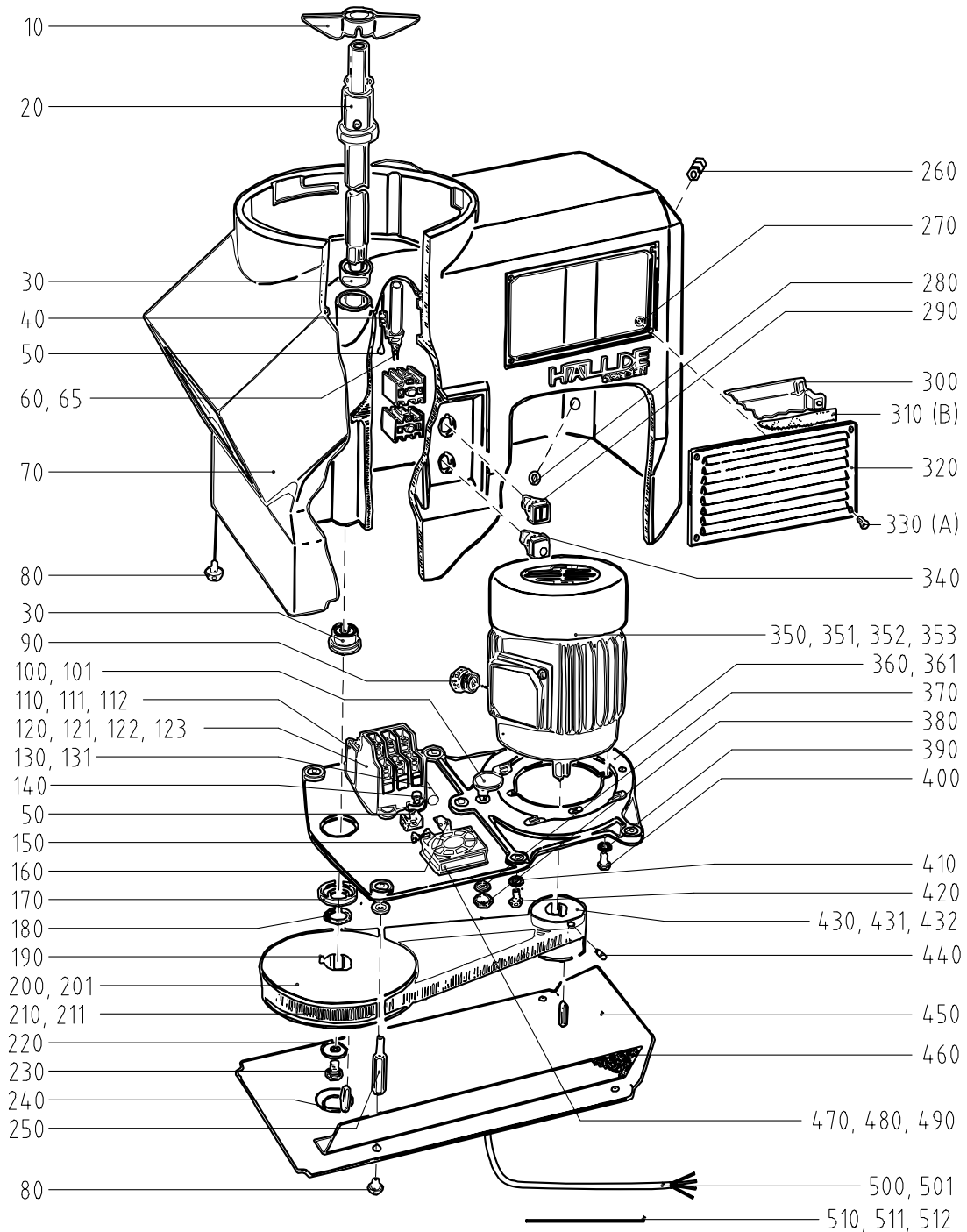
Drawing: Vegetable Preparation Machine RG-7
